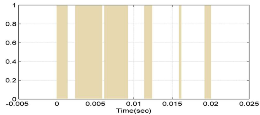
Figure 7. TR 2 gate signal.
