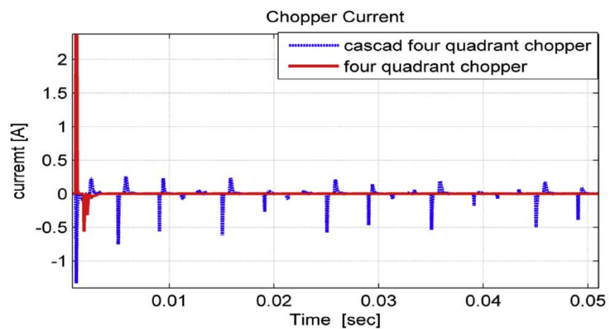
Figure 12. Chopper current.
