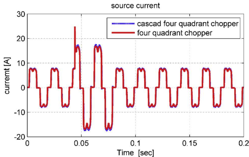
Figure 16. Source current in transient state.
