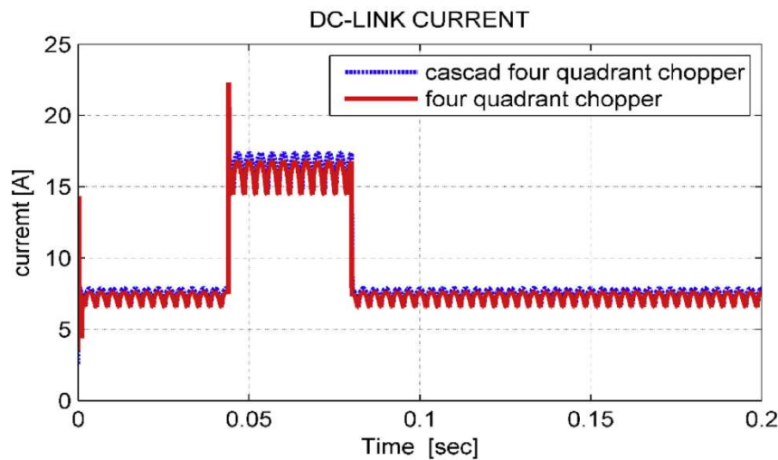
Figure 17. dc-link current in transient state.
