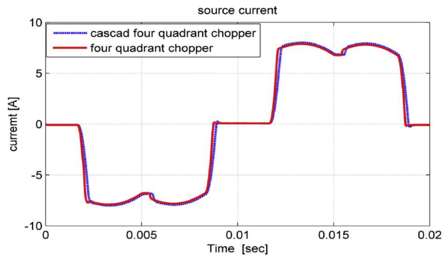
Figure 10. Grid currents.
