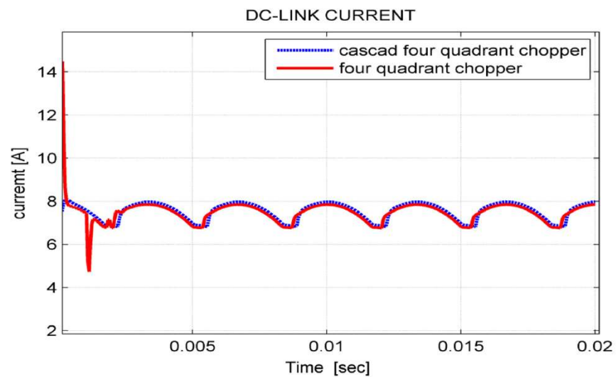
Figure 11. dc - link current.
