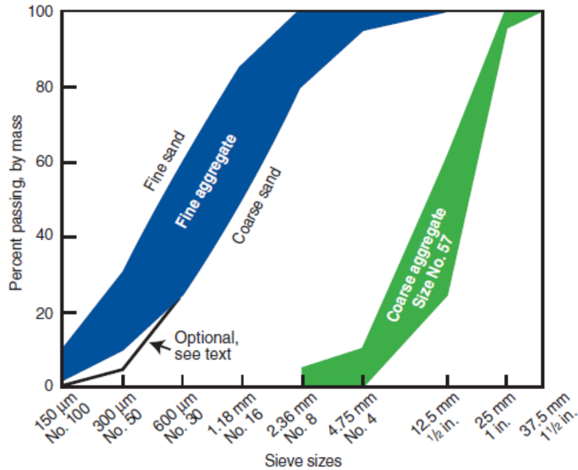
Curves indicate the limits specified in ASTM C 33
