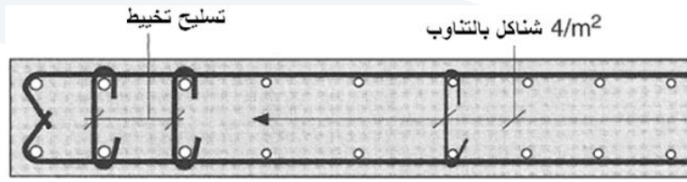
SEC. 2-2
