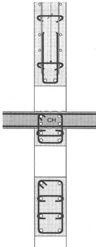
SEC. 3-3
