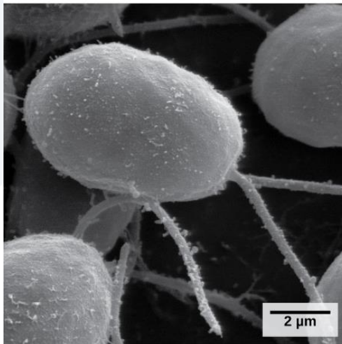
(c) Chlamydomonas
